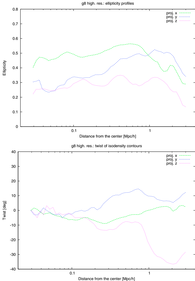
Fig. 4. Variations of ellipticity ( top panel ) and position angle ( bottom panel ) of the iso-density contours of the three projections of cluster g8_{hr} as function of the distance from the cluster centre. The cluster has a virial radius of \sim 2.7 h^{-1} \text{Mpc} .
