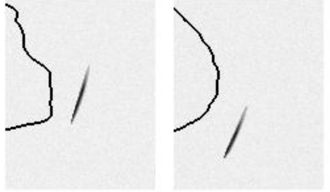
Fig. 15. Example of gravitational arc shifted by substructures. The size of the each frame is 27'' \times 34'' . Left panel: simulation including substructures. Right panel: simulation performed after smoothing with a smoothing length of 47 h^{-1} \text{kpc} .
