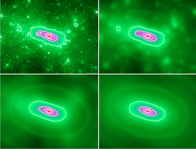
Fig. 2. Surface density maps of the same cluster projection as shown in Fig. 1, smoothed with increasing smoothing length from the top left to the bottom right panels. The background smoothed model is the one shown in the upper right panel of Fig. 1. The smoothing lengths in the four panels are 0, 47, 141 and 470 h^{-1} kpc comoving, respectively. The horizontal side length of each panel is 6 h^{-1} Mpc comoving.
