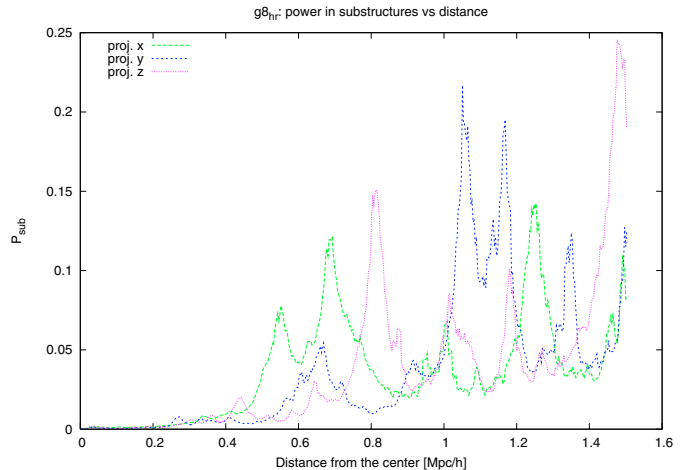
Fig. 5. Power in substructures as a function of distance from the cluster centre for the three projections along the x -, y - and z -axes of cluster g8_{hr} .
