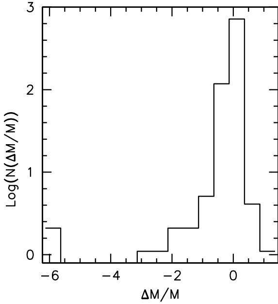
Fig. 18. Distribution of the relative variations of mass determinations from strong lensing, assuming axial symmetry and that the arc position trace the location of the critical lines.
