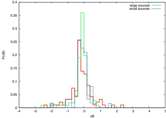
Fig. 16. Probability distribution function of the differences between arc magnitudes in simulation including and excluding substructures on scales <47 h^{-1} \text{kpc} . Results are shown for three different source sizes. See text for more details.
