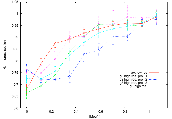
Fig. 13. Lensing cross section for arcs with length-to-width ratio larger than 7.5 as a function of the minimal equivalent radius containing substructures. Results are shown for all three cluster projections. The curves are normalised to the cross section of the cluster containing all its substructures, corresponding to l = \infty . The critical regions of the lenses have maximal radii in the range \sim 100\text{--}250 h^{-1}\text{kpc} .
