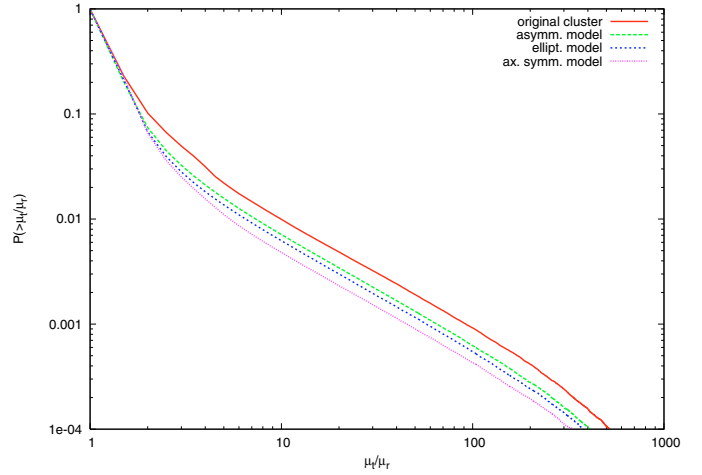
Fig. 7. Cumulative distributions of tangential-to-radial magnifications in the maps shown in Fig. 6.
