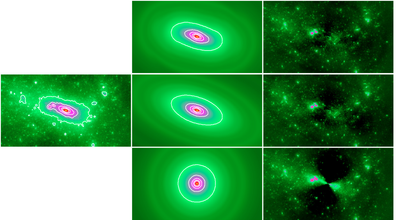
Fig. 1. Different smoothing sequences of the projection along the x -axis of cluster g8_{\text{hr}} . The original map is shown on the left. Top panels: smoothing with variable ellipticity and orientation of the iso-density contours; middle panels: smoothing assuming fixed ellipticity and position angle (see text for more details); bottom panels: smoothing assuming axial symmetry. From left to right, each row of panels show the smoothed map and the residuals, obtained by subtracting the smoothed from the original map. The contour levels in the density maps start at \sim 3.6 \times 10^{15} h M_{\odot} \text{Mpc}^{-2} and are spaced by 5 \times 10^{15} h M_{\odot} \text{Mpc}^{-2} . The horizontal side length of each panel is 6 h^{-1} \text{Mpc} .
