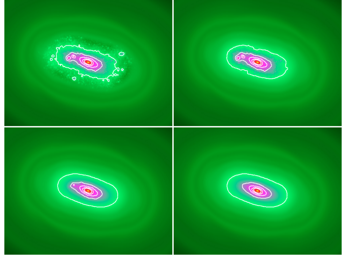
Fig. 3. Surface density maps of the same cluster projection shown in Fig. 1, suppressing the substructures in shells of decreasing equivalent radius from the top left to the bottom right panels. The background smoothed model is the one shown in the upper right panel of Fig. 1. The equivalent radii beyond which the substructures are removed are 1174, 704, 352 and 235 h^{-1} kpc comoving, respectively. The horizontal side length of each panel is 6 h^{-1} Mpc comoving.
