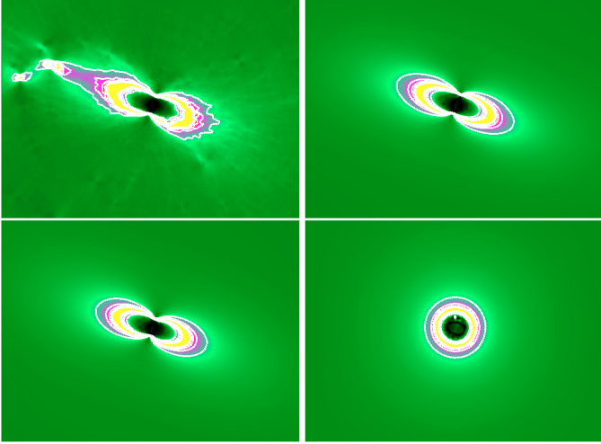
Fig. 6. Maps of the tangential-to-radial magnification ratio for the same cluster projection showed in the previous figures. From the top left to the bottom right panel, we show the maps corresponding to the original cluster and to three smoothed versions of it: using the asymmetric, the elliptical and the axially symmetric background models.
