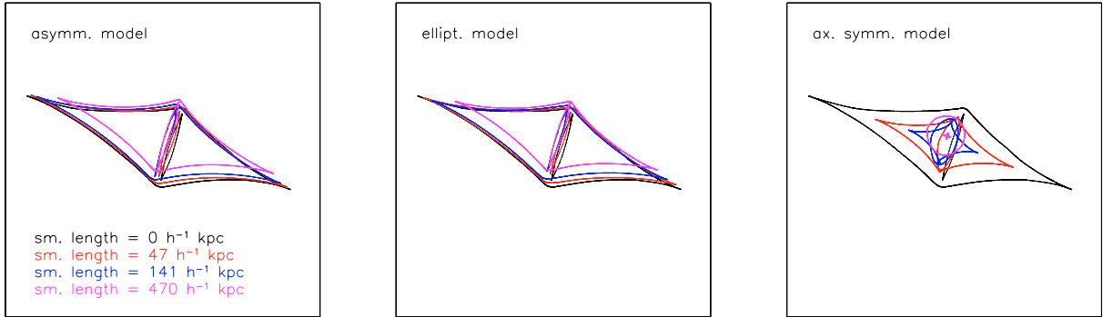
Fig. 8. Lens caustics of the mass distribution of the cluster projected along the x -axis as obtained after smoothing using several smoothing lengths and assuming different background models: asymmetric model ( left panel ), elliptical model ( central panel ) and axially symmetric model ( right panel ). The side length of each panel is 500 h^{-1} \text{ kpc} comoving, corresponding to \sim 1' .
