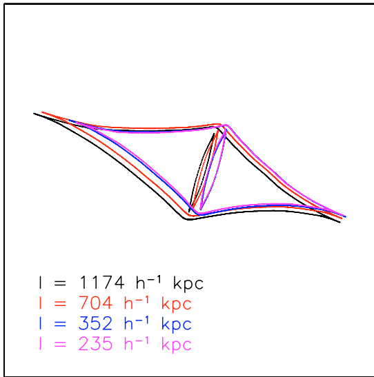
Fig. 9. Lens' caustics obtained after removing substructures from the region outside a given radius, as given by the labels in the figure. The side length is 500 h^{-1} \text{ kpc} comoving, corresponding to \sim 1' . The figure refers to the cluster projection along the x axis.
