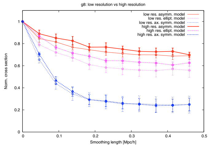
Fig. 11. Comparison between the low and the high resolution version of cluster g8 . The lensing cross section for arcs with length-to-width ratio larger than 7.5 averaged over three orthogonal projections of the same cluster are plotted versus the smoothing function.
