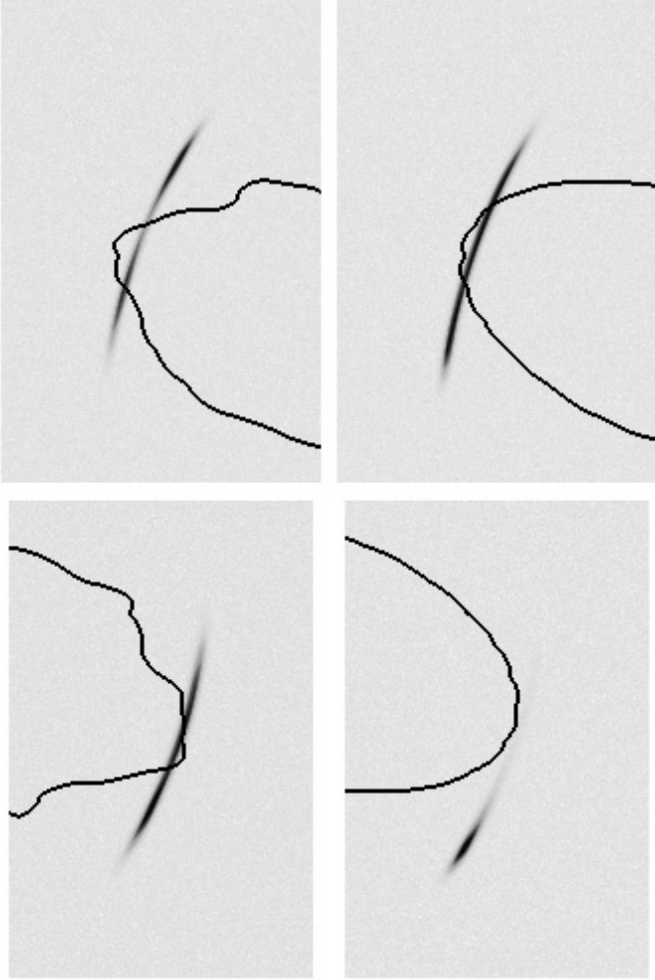
Fig. 14. Effects of substructures on scales \lesssim 50 h^{-1} \text{kpc} on the morphology of gravitational arcs. In the left panels shown are the arcs formed out of two different sources lensed by the unsmoothed mass distribution displayed in the top left panel of Fig. 2. In the right panels, shown are the corresponding images obtained by using as lens the mass distribution given in the top right panel of Fig. 2, which has been obtained by smoothing with a smoothing length of 47 h^{-1} \text{kpc} . In all panels, the critical lines are drawn for comparison. The top and the bottom panels have sizes of 38'' \times 57'' and 36'' \times 56'' , respectively.
