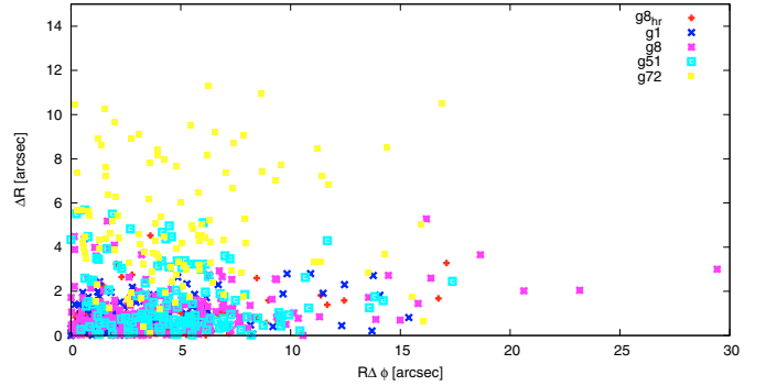
Fig. 17. Distribution of long arcs (length >5'' ) in the plane radial ( \Delta R ) vs. tangential ( R\Delta\phi ) shift. Different symbols identify arcs produced by different clusters. The arcs produced by the cluster g72 , which is experiencing a major merger, are given by the small filled squares.
