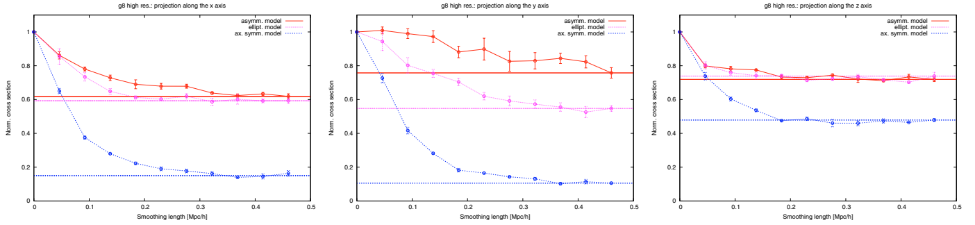
Fig. 10. Lensing cross section for arcs with length-to-width ratio larger than 7.5 as a function of the smoothing length. Solid, dashed and dotted lines refer to smoothing adopting the asymmetric, the elliptical and the axially symmetric background models, respectively. The curves are normalised to the corresponding cross section for smoothing length equal to zero. The results are shown for the cluster projections along the x - (left panel), y - (central panel), and z -axes (right panel). The critical lines in the three projections are contained in rectangles sized (395 \times 105) h^{-2} \text{kpc}^2 , (455 \times 205) h^{-2} \text{kpc}^2 and (262 \times 87) h^{-2} \text{kpc}^2 , respectively.
