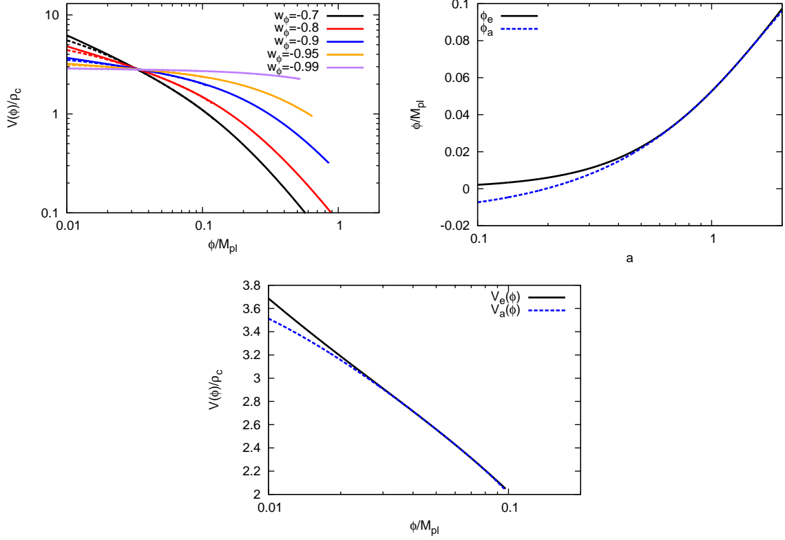
FIG. 3. Left panel : Approximation of the scalar field potential for a \approx 1 for different constant equation-of-state parameters w_\phi . Solid lines represent the exact numerical solution, while the dashed line show the approximated solution. Colours are as in Figure 1 . Middle (right) panel : scalar field (potential) for the approximated solution compared with the exact expression (41) together with (46) for w_\phi = -0.9 . In all the panels we assume G(\chi) = -\frac{\chi}{M^4} + \frac{\chi^2}{M^8} .
