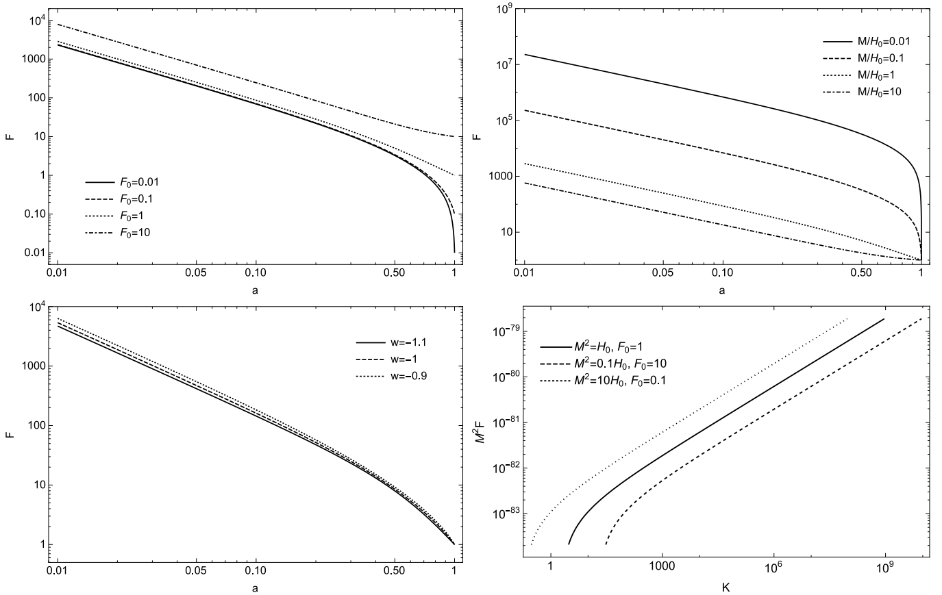
FIG. 1. Top left panel: Comparison of the evolution of \mathcal{F} due to varying \mathcal{F}_0 . In these models M = H_0 and w_{\text{de}} = -1 are fixed. Top right panel: Comparison of the evolution of \mathcal{F} due to the variation of M , as a multiple of H_0 . In these models \mathcal{F}_0 = 1 and w_{\text{de}} = -1 are fixed. Bottom left panel: Comparison of the evolution of \mathcal{F} for varying w_{\text{de}} close to -1 . In these models \mathcal{F}_0 = 1 and M = H_0 are fixed. Bottom right panel: Comparison of the evolution of M^2 \mathcal{F} for varying M^2 and \mathcal{F}_0 , with M^2 \mathcal{F}_0 / H_0^2 = 1 and w_{\text{de}} = -1 fixed.
