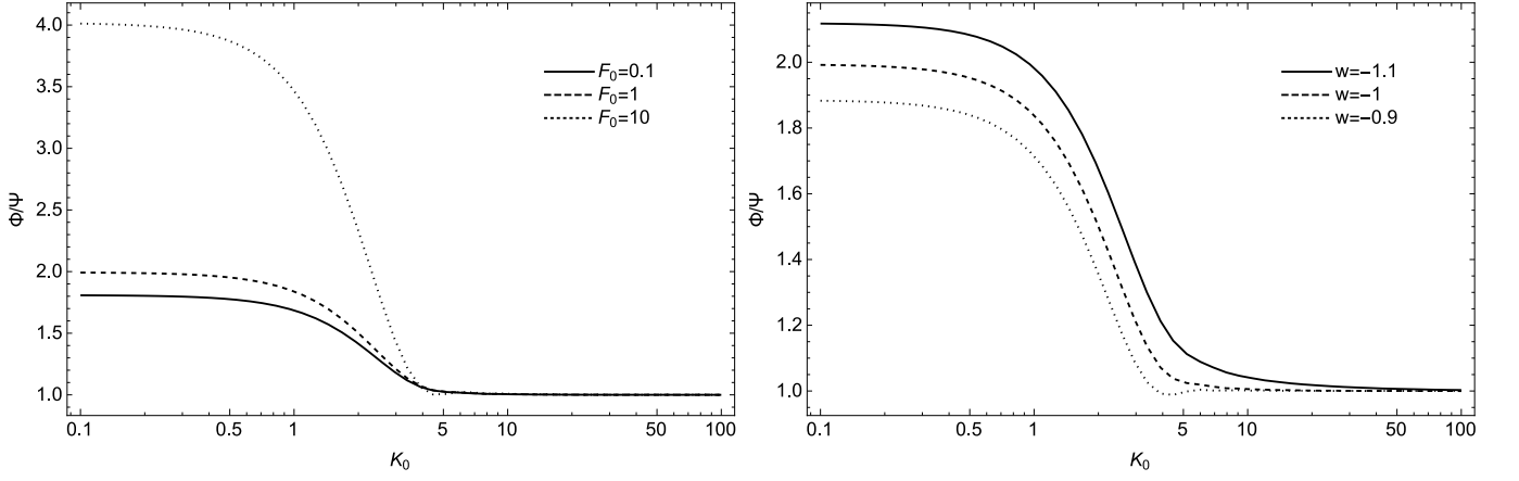
FIG. 2. Left panel: The spectrum of \Phi/\Psi , or Z/Y , at a = 1 as a function of scale for varying \mathcal{F}_0 and w_{\text{de}} = -1 . Right panel: The spectrum of \Phi/\Psi at a = 1 as a function of scale for a General Einstein-Aether fluid with w_{\text{de}} varying around -1 and \mathcal{F}_0 = 1 .
