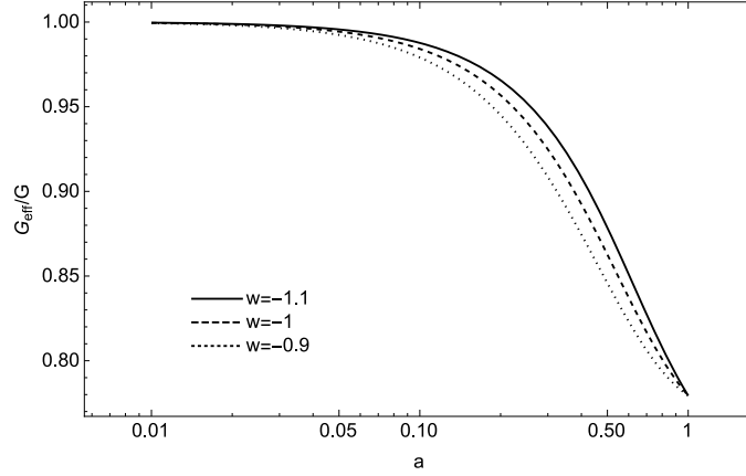
FIG. 3. The evolution of the effective Newton's constant, G_{\text{eff}}/G , is shown for varying w_{\text{de}} around -1 .
