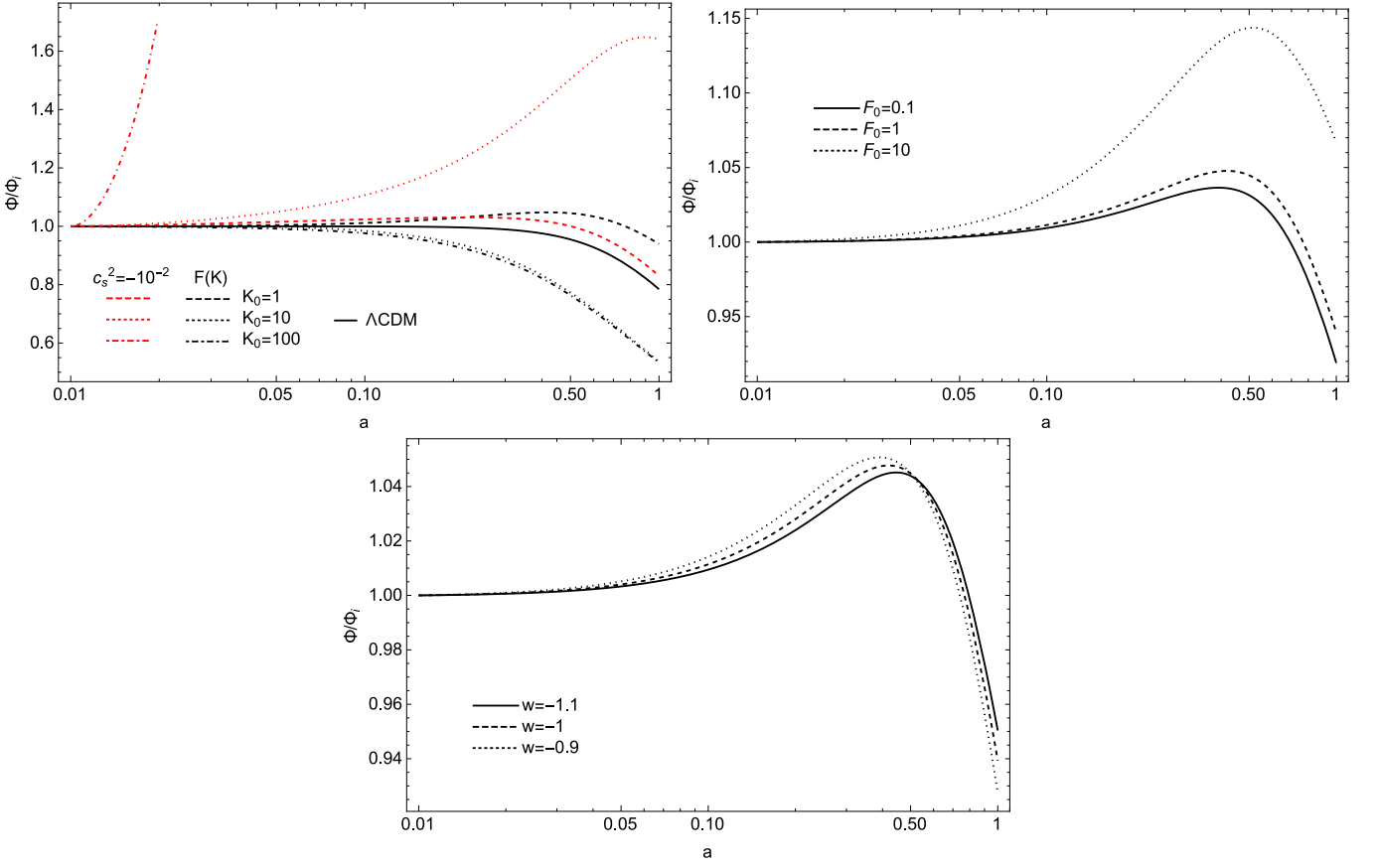
FIG. 4. Top left panel: The evolution of the Newtonian potential, \Phi , in \Lambda CDM (black solid line) and for different scales in a designer \mathcal{F}(\mathcal{K}) model (dashed and dotted lines) for \mathcal{F}_0 = 1 and w_{\text{de}} = -1 . Note that the potential for the \Lambda CDM model is scale independent. For comparison we also show the evolution of \Phi with the presence of a dark energy fluid with w_{\text{de}} = -1 and a constant negative squared sound speed of c_s^2 = -10^{-2} (red lines), calculated using (144). Top right panel: The evolution of \Phi in a Generalized Einstein-Aether universe with varying \mathcal{F}_0 for w_{\text{de}} = -1 and K_0 = 1 fixed. Bottom panel: The evolution of \Phi for a General Einstein-Aether fluid with w_{\text{de}} varying around -1 , with \mathcal{F}_0 = 1 and K_0 = 1 fixed.
