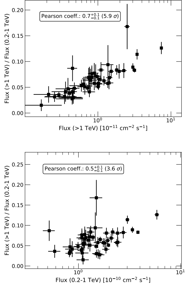
Fig. 3: Hardness ratio ( F_{>1 \text{ TeV}} / F_{0.2-1 \text{ TeV}} ) versus F_{>1 \text{ TeV}} (top figure) and versus F_{0.2-1 \text{ TeV}} (lower figure) from the MAGIC measurements. The Pearson's coefficients and the corresponding significance (following the prescription of Press et al. 2007) are given in both plots.
