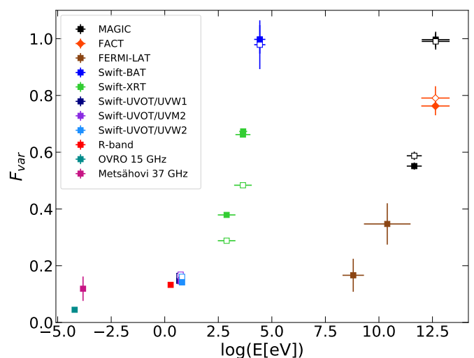
Fig. 6: Fractional variability F_{var} obtained from the light curves shown in Fig. 1. MAGIC, FACT, Swift -XRT, Swift -UVOT, R-band and radio fluxes are nightly binned. Fermi -LAT and Swift -BAT fluxes have a 3-day binning. Results from each instrument are plotted in different colours. The filled markers include all data. The hollow markers include VHE and Swift data lying within a time window of 4 hours from each other.
