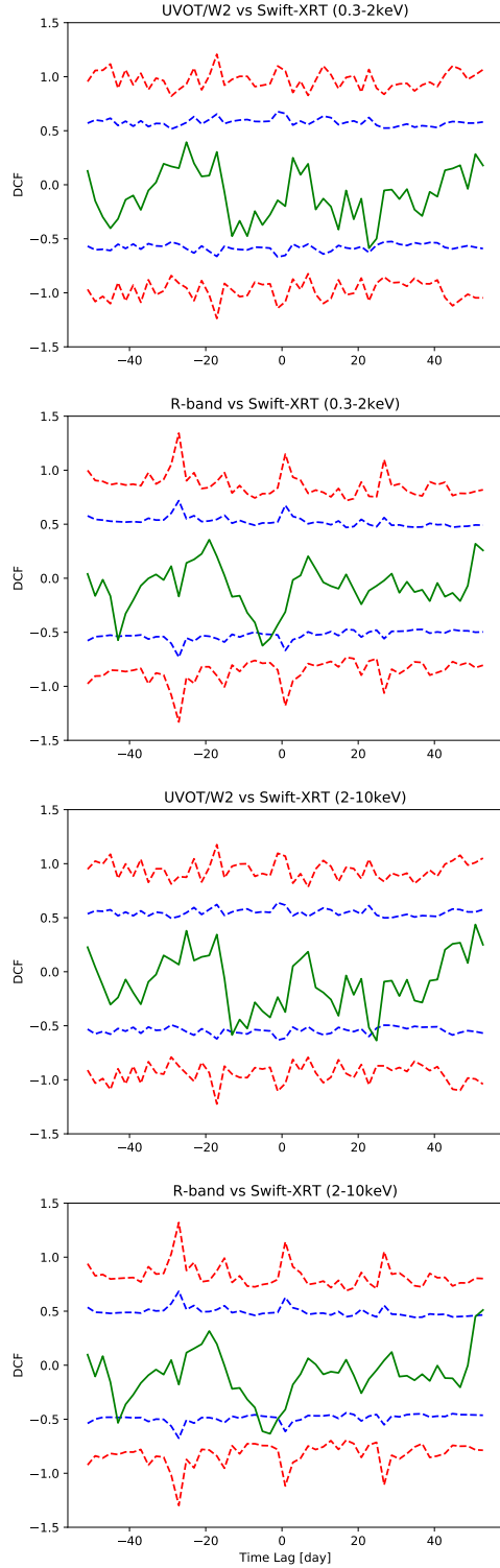
Fig. F.1: DCF between X-ray (0.3-2 keV and 2-10 keV) and UV/optical (Swift-UVW2 and R-band) when removing data before MJD 57760. The blue- and red-dashed-lines indicate the 2\sigma and 3\sigma confidence intervals estimated from the Monte Carlo simulations, as described in the text.
