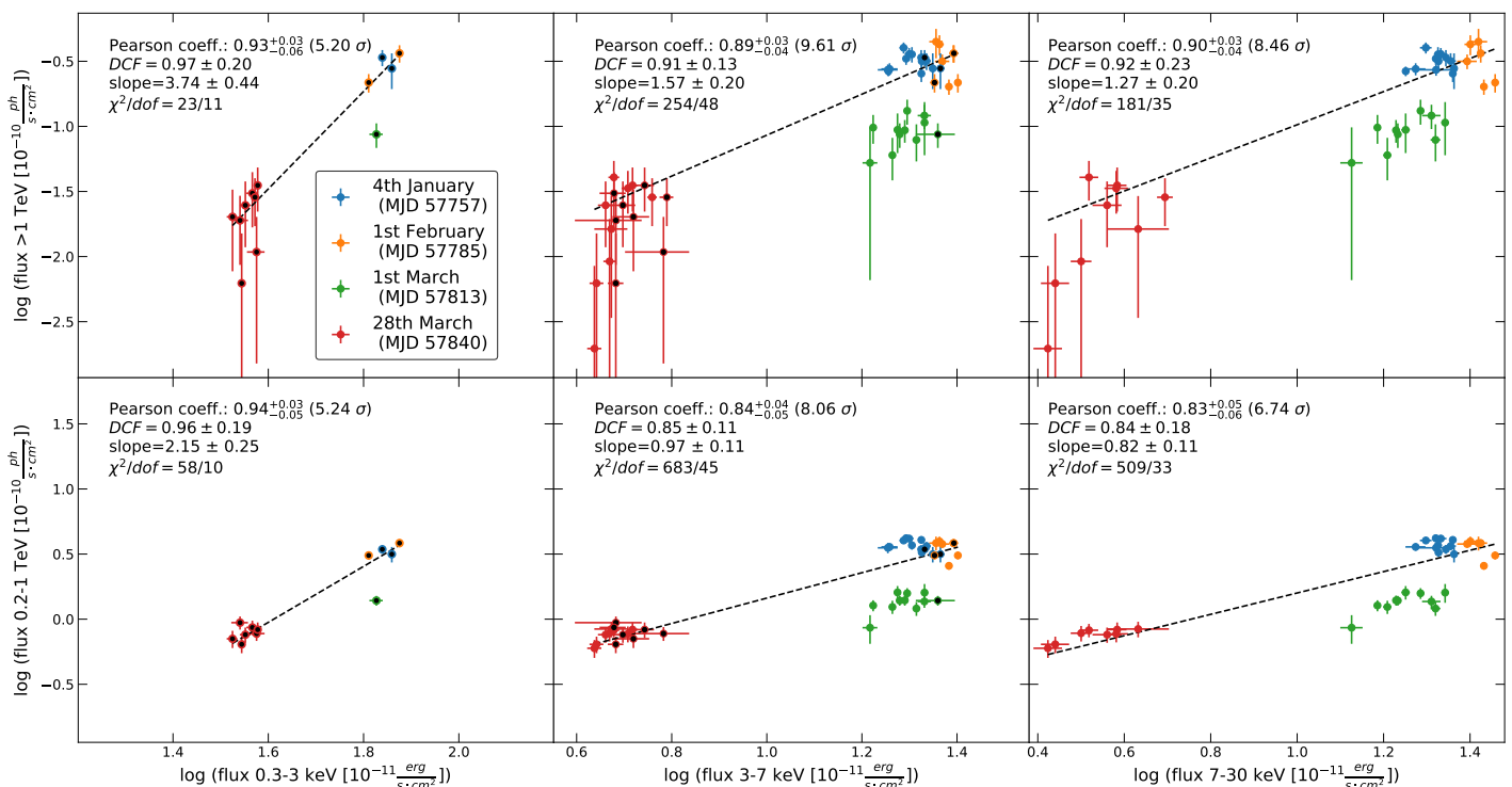
Fig. 8: VHE flux versus X-ray flux during the simultaneous MAGIC/NuSTAR/Swift observations. Flux points are computed over time bins of 30 minutes. From left to right, the X-ray energy bands in the panels are 0.3-3 keV, 3-7 keV and 7-30 keV. In the upper panels, the MAGIC fluxes are in the >1 TeV band, while in the lower panels they are in the 0.2-1 TeV band. Data points from Swift-XRT are shown with black-filled markers. Fluxes corresponding to each day are plotted in a different colour. The results of the Pearson coefficients (and its significance in \sigma ), DCF and the slope of the linear fits in the log-log plane (with the \chi^2/dof values) are indicated in each of the corresponding subplots.
