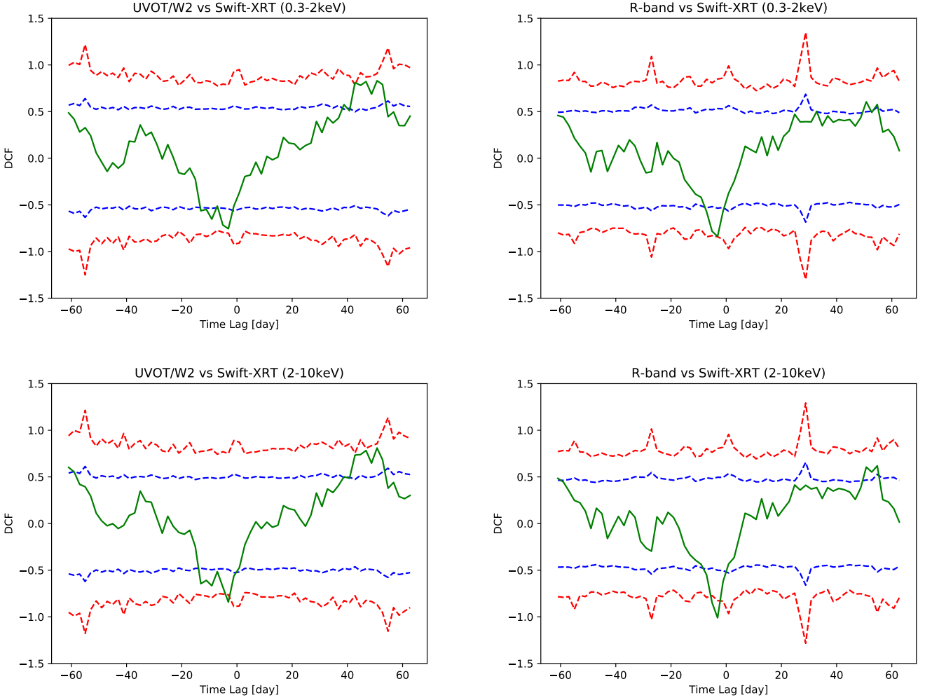
Fig. 14: DCF between X-ray (0.3-2 keV and 2-10 keV) and UV/optical ( Swift -UVW2 and R-band) during the MWL campaign. The blue- and red-dashed-lines indicate the 2\sigma and 3\sigma confidence intervals estimated from the Monte Carlo simulations, as described in the text.
