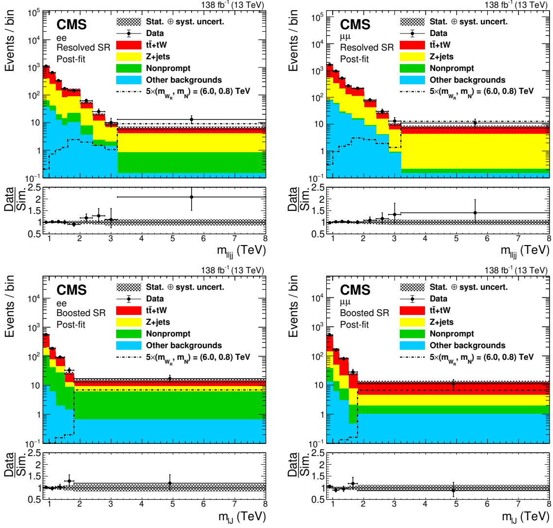
Figure 5. The background-only post-fit m_{\ell\ell jj} ( m_{\ell j} ) distributions in the resolved (boosted) SR are shown in the upper (lower) plot. Results for the dielectron (dimuon) channel are shown on the left (right). Statistical and systematic uncertainties in the expected background yields are represented by the hatched band. The simulated signal distribution is scaled up by a factor of five to enhance visibility.
