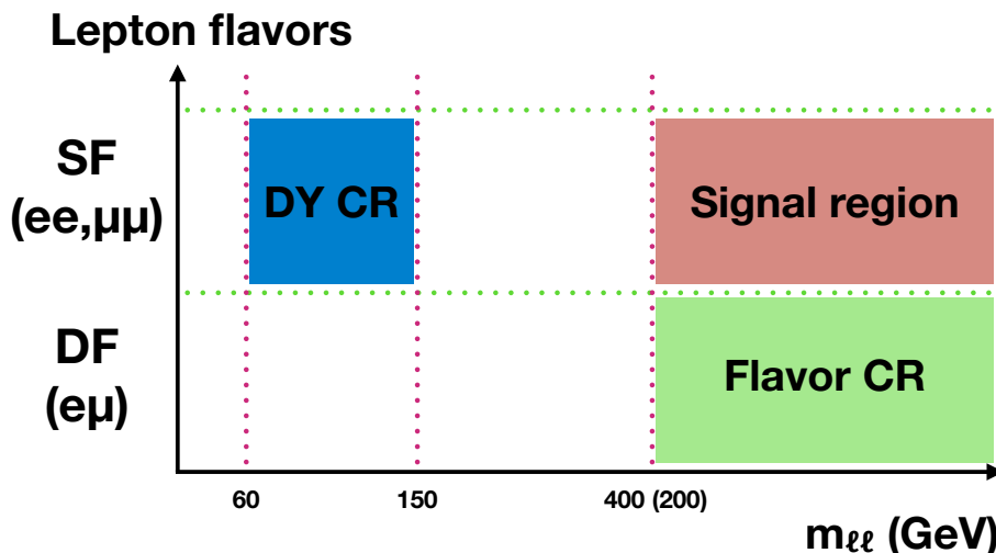
Figure 2. A schematic diagram of the analysis region. The minimum values of the dilepton mass in the SR and the flavor CR is 400 (200) GeV for the resolved (boosted) region. The backgrounds from tW and t\bar{t} production are estimated from the flavor CR (green), where different flavor (DF) leptons are required. The DY background is estimated from the DY CR (blue).
