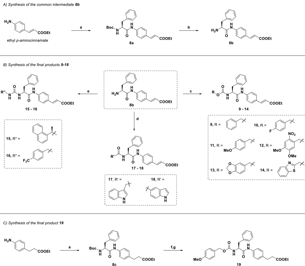
Scheme 1 Synthesis of 9–19. Reagents and conditions: (a) Boc-Phe-OH, EDCI, HOBT, dry DMF, rt, overnight, 84–49%; (b) TFA, dry DCM, rt, 4 h, then K_2CO_3 , 91%; (c) 4- NO_2PhOCO_2R , DIPEA, dry THF, 0 °C to rt, overnight, 32–68%; (d) R'CO_2H , EDCI, HOBT, dry DMF, rt, overnight, 31–45%; (e) R''NCO , NEt_3 , dry THF, 0 °C to rt, overnight, 60–88%. (f) TFA, dry DCM, rt, 4 h, quant. yield; (g) 4-methoxybenzyl (4-nitrophenyl) carbonate, DIPEA, dry THF, rt, overnight, 38%.
