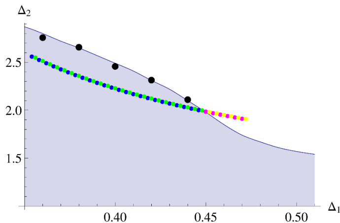
Figure 6. Plot of the one-parameter family of the truncation (4,3,0) in the plane (\hat{\Delta}_1, \hat{\Delta}_2) , superimposed to the upper unitarity bound found in [14]. The blue and green dots correspond respectively to the minimal and the maximal choice of the pair (\Delta_{\varepsilon''}, \Delta_{\varepsilon'''}) , as determined in figure 4. These dots are replaced by ones respectively magenta and yellow when some OPE coefficient become negative. For the black dots on the unitarity bound see explanation in the text.
