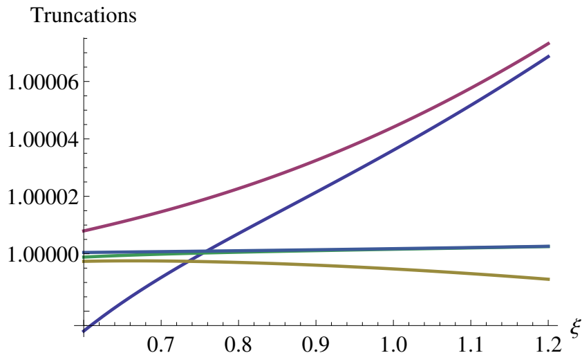
Figure 2. The left-hand-side of the sum rule (2.9) for various truncations (n_{\text{bulk}}, n_{\text{bdy}}, 0) of the two-point function of the 2d Ising model in the ordinary transition. Only in the n_{\text{bulk}} \rightarrow \infty , n_{\text{bdy}} \rightarrow \infty limit the sum rule is saturated.
