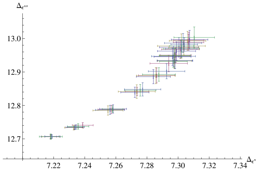
Figure 4. Parametric plot of the scaling dimensions of \Delta_{\varepsilon''} and \Delta_{\varepsilon'''} generated by the unknown parameter \hat{\Delta} . Here we see the effect of the statistical errors on the input data, namely \Delta_{\sigma} , \Delta_{\varepsilon} and \Delta_{\varepsilon'} as well as the effect of the spread of the solutions. Some of these data are presented in table 3.
