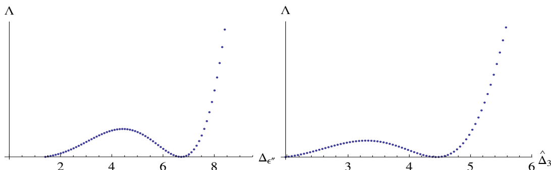
Figure 7. Linear functionals for the bulk and boundary channels in the special transition.
