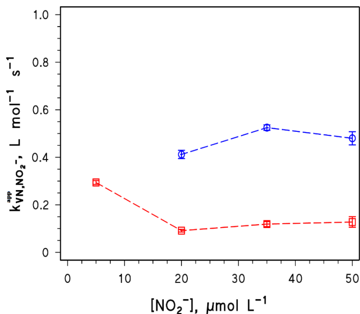
Fig.SI-8. Apparent second-order rate constant of VN photodegradation mediated by nitrite in artificial snow. The blue data refer to 5 μmol L -1 as initial VN concentration, while the red ones to 50 μmol L -1 VN.
