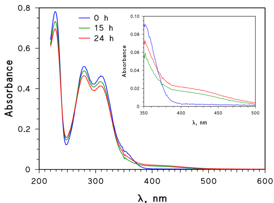
Fig.SI-9. Absorption spectra of (melted) artificial snow samples recorded before and after 15 - 24 h of UVA irradiation. The initial chemical composition of snow was 50 μmol L -1 NO 2 - , 50 μmol L -1 VN and 16.7 μmol L -1 Na 2 SO 4 . The inset shows the increase of absorbance for λ > 380 nm after irradiation.
