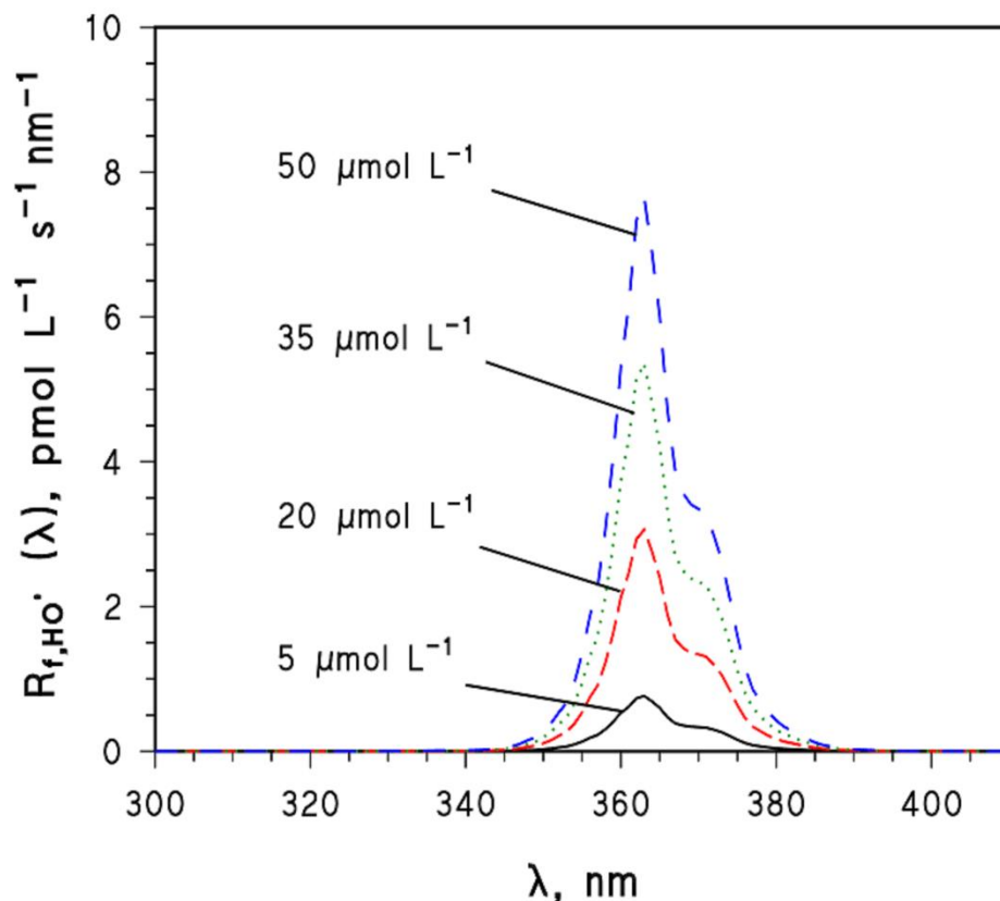
Fig.SI-7. Spectral photoproduction rate of hydroxyl radicals in the irradiated snow samples, at different concentrations of nitrite. Note that the total rate of \text{HO}^{\bullet} formation is the integral of each curve.
