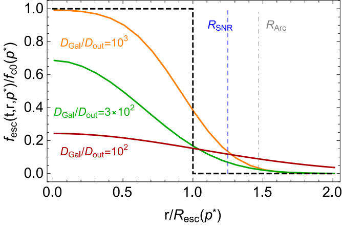
Fig. 6. Distribution of escaping particles at p^* = 10 TeV/c and t = t_{\text{SNR}} as a function of the radial coordinate normalised to R_{\text{esc}}(p^*) = 13 pc. Different lines refer to different values of the diffusion coefficient, as labelled. The vertical lines correspond to the shock position (dashed) and to the arc external edge (dot-dashed) as observed now. The remaining parameters are the same as in figure 5.
