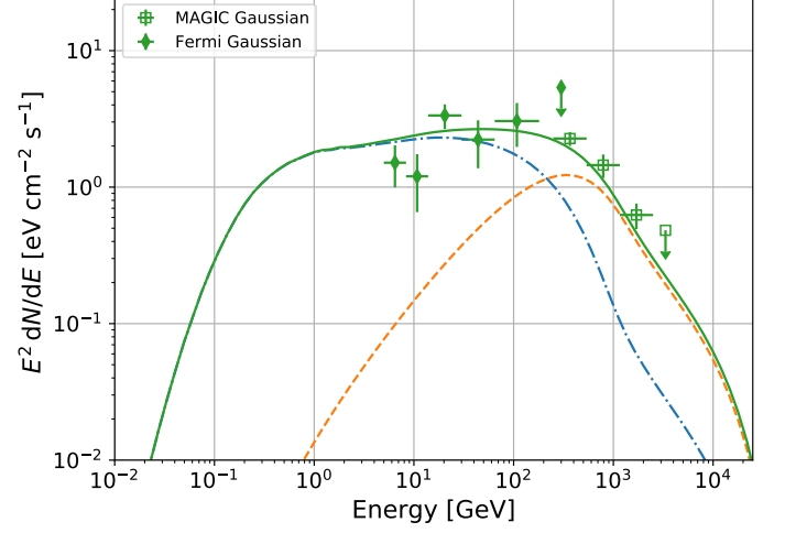
Fig. 9. Computed \gamma -ray flux due to \pi^0 decay from MAGIC J2019+408 based on our model compared against data points from our Fermi -LAT (diamonds) and the MAGIC (squares) analysis. The spectrum (solid, green line) is modelled as the sum of emission from the remnant interior (blue dash-dotted line) and exterior (orange dashed line).
