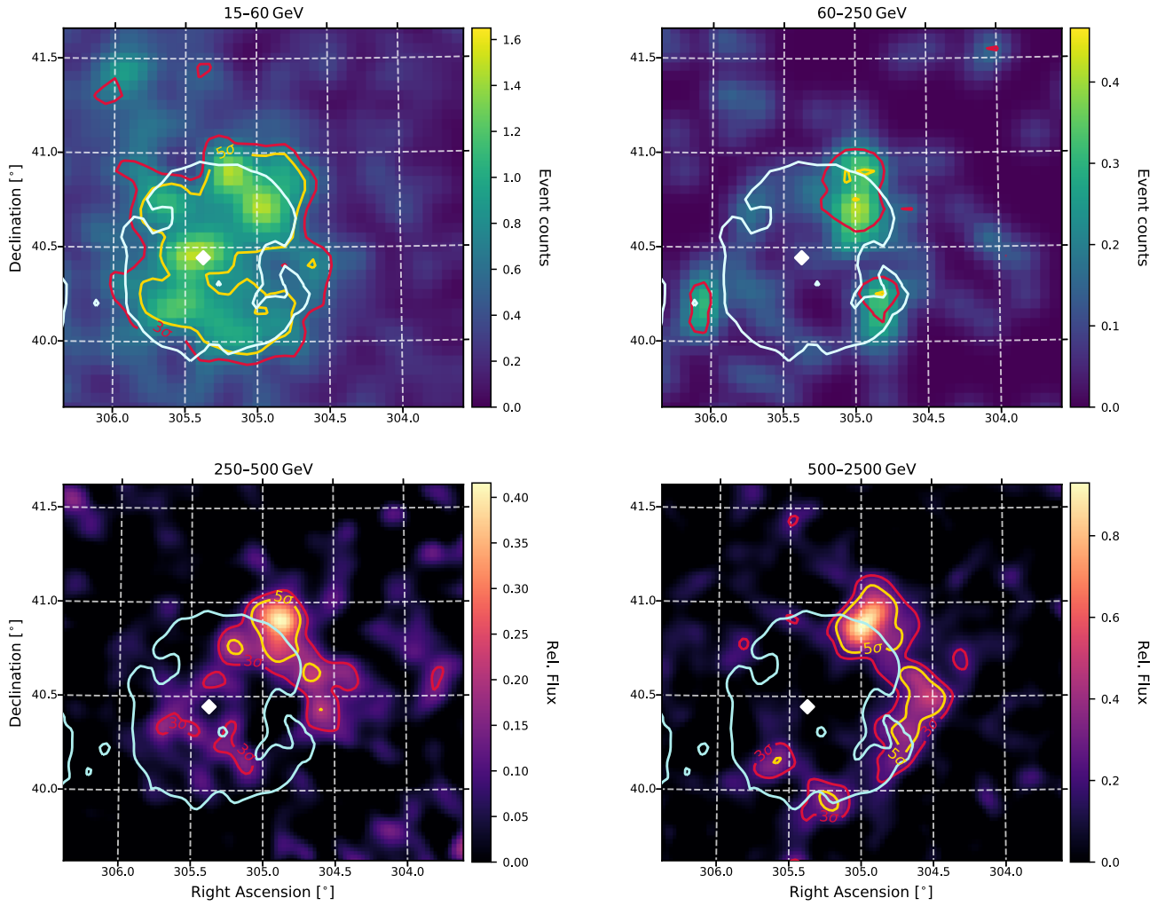
Fig. 2. Energy-dependent morphology of the \gamma -Cygni SNR. Upper left: Fermi -LAT count map between 15 and 60 GeV smoothed with a Gaussian kernel ( \sigma = 0.75 ) and 3 and 5 \sigma contours of a point source search. The white line is the 400 K contour of the 408 MHz observation by the CGPS. The white diamond identifies the position of PSR 2021+4026. Upper right: same as upper left but in the range from 60 and 250 GeV. Lower left: relative flux map observed by MAGIC at 250 to 500 GeV together with 3 and 5 \sigma point source significance contours. The same radio contours as in upper panels are displayed in cyan. Lower right: same as lower left but in the energy range from 500 GeV to 2.5 TeV.
