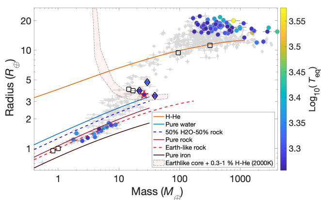
Fig. 10: Diagram of all known planets with masses from radial velocity measurements up to 13 M_J and radii from transit photometry with 30 % and 10 % uncertainties or lower in mass and radius, respectively. Planets with T_{\text{eq}} \geq 1800 K are colour-coded with T_{\text{eq}} , and the rest are plotted in light grey. In total, there are four planets (including TOI-2196 b) with radii between 3 and 5 R_{\oplus} in this diagram that are identified as hot Neptune desert planets (cf. Fig. 9). TOI-2196 b is marked with a red star symbol and the three additional planets with black diamonds. Solar system planets are marked with brown squares. Interior models from Zeng et al. (2019) are plotted as listed in the legend. The 100 % water line is for a planet with condensed water phases.
