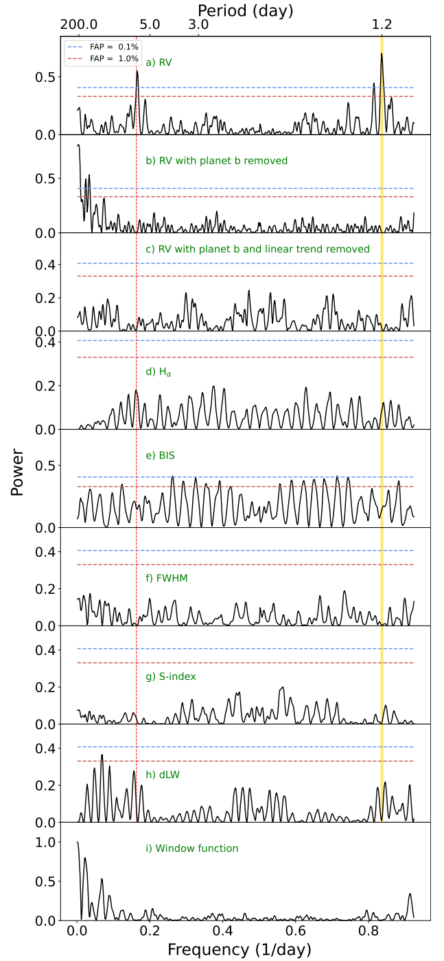
Fig. 4: Generalised Lomb-Scargle periodogram of the HARPS RVs and stellar activity indicators. The horizontal lines mark the bootstrap false alarm probabilities at 0.1 and 1.0 % as indicated in the legend. The orbital frequency of TOI-2196 b ( \nu_b = 0.837 \text{ day}^{-1} ) is marked with a vertical thick yellow line, while the corresponding period is reported in the upper x-axis ( P_{\text{orb}} \approx 1.2 \text{ day} ). The 1 day alias of planet b is marked with a vertical dashed red line ( 1 - 0.837 = 0.163 \text{ day}^{-1} ). a) RV measurements. b) RV residuals with the best-fitting Keplerian orbit of planet b subtracted. c) RV residuals following the subtraction of both the linear trend and the Doppler signal induced by planet b. d-h) Activity indicators and line profile variations. i) The window function.
