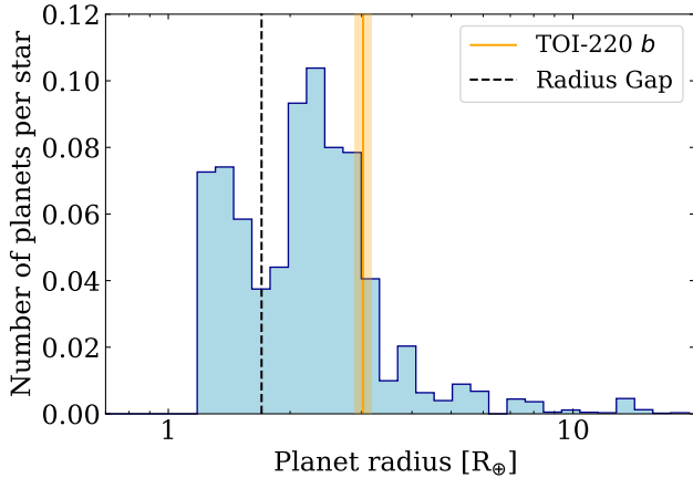
Figure 12. Histogram of the planetary radius for planets with periods below 100 d as presented in Fulton & Petigura (2018). The location of the radius gap and the size of TOI-220 b ( \pm 1 \sigma ) are shown with the black-dashed and orange-shaded lines, respectively.
