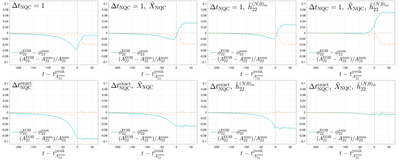
FIG. 6. Analytical/numerical differences for the amplitude and the phase (in radians) of the quadrupolar waveform for the quasi-circular inspiral-plunge in Schwarzschild. We consider different inspiral-plunge and ringdown matching procedures. The differences are shown from the LSO crossing to t_{A_{22}}^{\text{peak}} + 70 . In the upper panels we consider the matching time according to Eq. (27), while in the lower panels we use Eq. (28). Then, from left to right, we progressively improve the model considering the second time derivatives in the NQC base, \ddot{X}_{22} and \ddot{\omega}_{22} , and then the Newtonian noncircular correction, \hat{h}_{\ell m}^{(N,0)\text{nc}} . The rightmost lower panel shows the differences for the state-of-the-art model.
