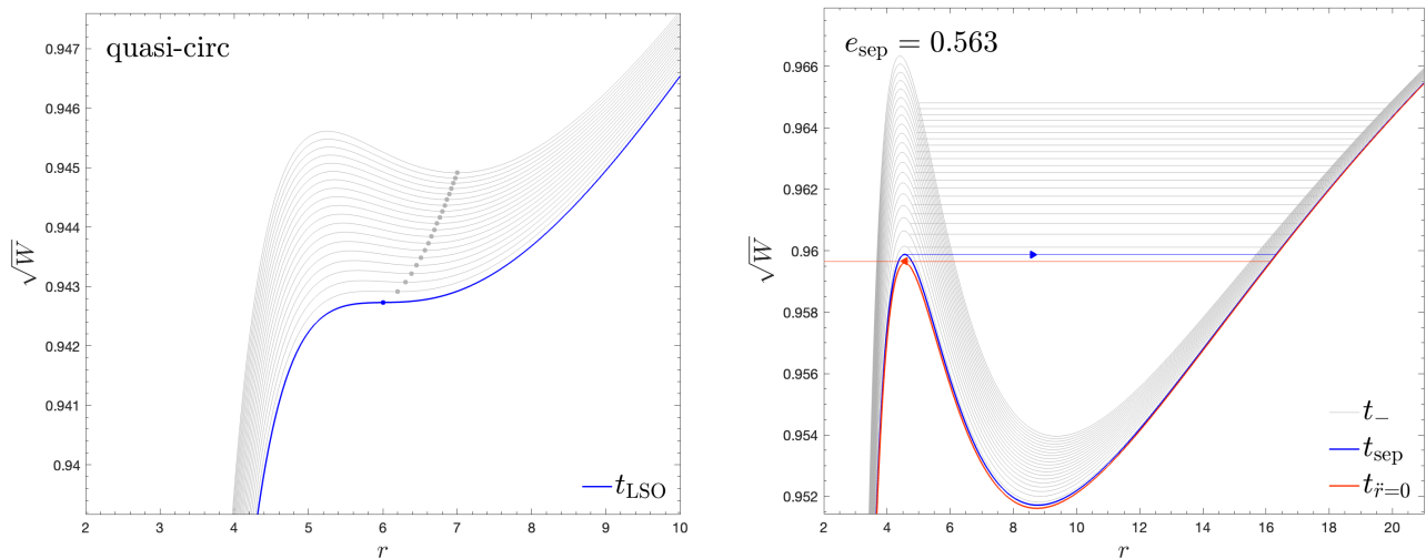
FIG. 1. Left panel: the evolution of radial effective potential W , Eq. (7), along the transition from quasi-circular inspiral up to the Last Stable Orbit. The LSO potential is highlighted, while the minima (identified by visible markers) indicate the radius and energy of the particle. Right panel: eccentric case with initial eccentricity e_0 = 0.6 ( e_{\text{sep}} = 0.563 ). We show a sequence of potentials W (that change due to radiation reaction) and corresponding energies of the particle at the periastron (horizontal line, gray) during the bound motion of the inspiral. The quantities at the separatrix crossing are shown in blue, while the red lines correspond to the beginning of the plunge. Note that in this case one has V_{\text{max}} \lesssim E . The horizontal arrows mark the radial location (and energy) of the particle along the orbit at t = t_{\text{sep}} and at t = t_{\dot{r}=0} . Note that the arrows point toward the corresponding direction of the radial motion, outgoing for t = t_{\text{sep}} and ingoing for t = t_{\dot{r}=0} . This latter point can be considered a missed periastron and practically marks the beginning of the plunge.
