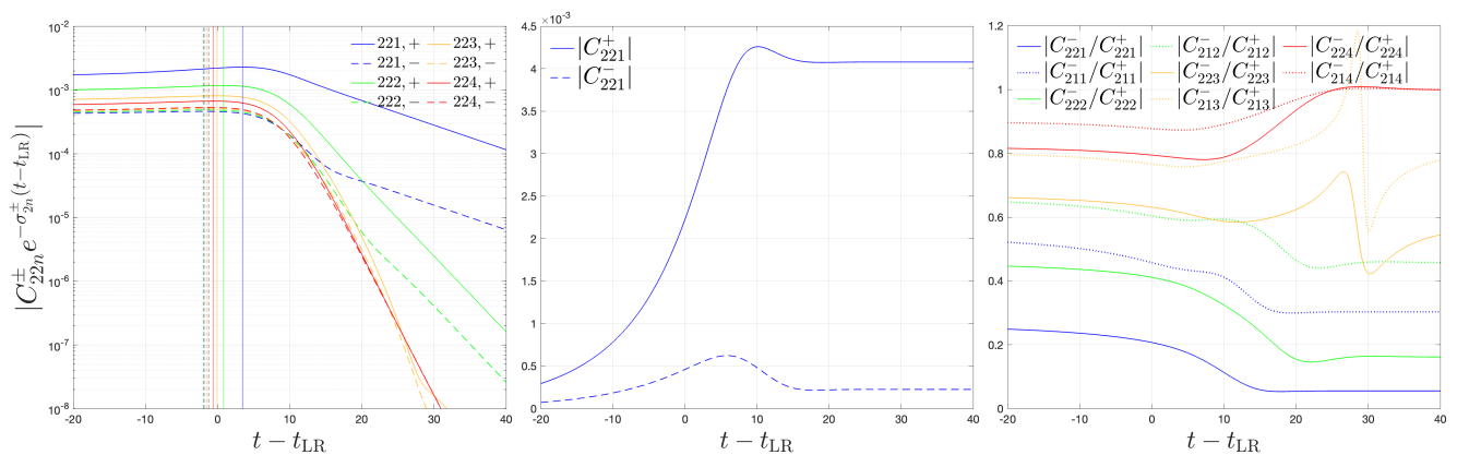
FIG. 20. Time-dependent QNM-excitation coefficients C_{\ell mn}^{\pm}(t) for the quasi-circular case, see Eq. (53). The positive-frequency modes are more relevant and are excited later than the negative ones, as shown by the location of the amplitude maxima (vertical lines in the leftmost plot). In the middle panel we plot the activation-like excitation coefficients for the fundamental frequency. The rightmost panel highlights the hierarchy of the ratios |C_{\ell mn}^{-}/C_{\ell mn}^{+}| for the overtones of the (2,2) and (2,1) multipoles. Note that the beating is more relevant for the (2,1) mode (dotted line) than for the quadrupole (solid lines).
