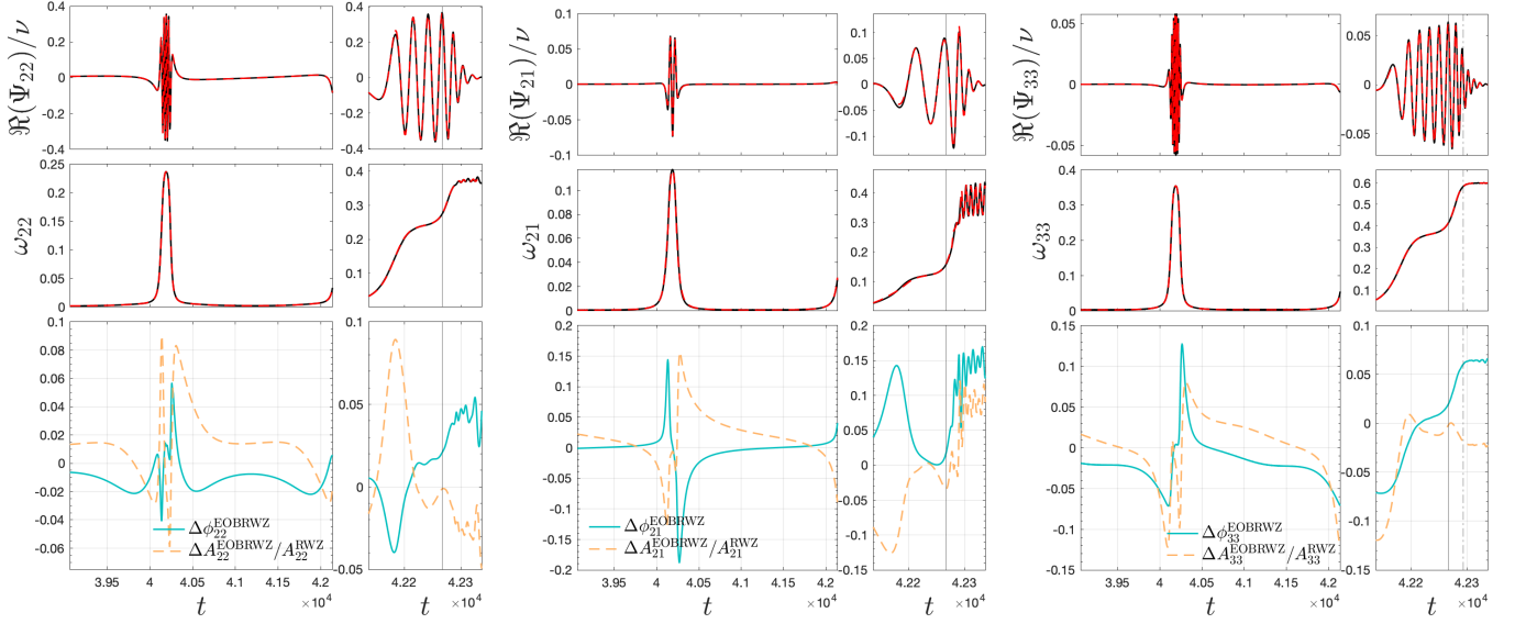
FIG. 11. Analytical/numerical comparisons for the (2,2), (2,1) and (3,3) multipoles for the configuration with initial eccentricity e_0 = 0.95 . We show the real part and the frequency of the RWZ waveform (black) and the complete EOB waveform (red, dashed). In the bottom panels we show the relative amplitude difference (orange dashed) and the phase difference in radians (light blue). The vertical solid lines mark the peak of A_{22} , while the dash-dotted ones mark t_{A_{\ell m}}^{\text{peak}} .
