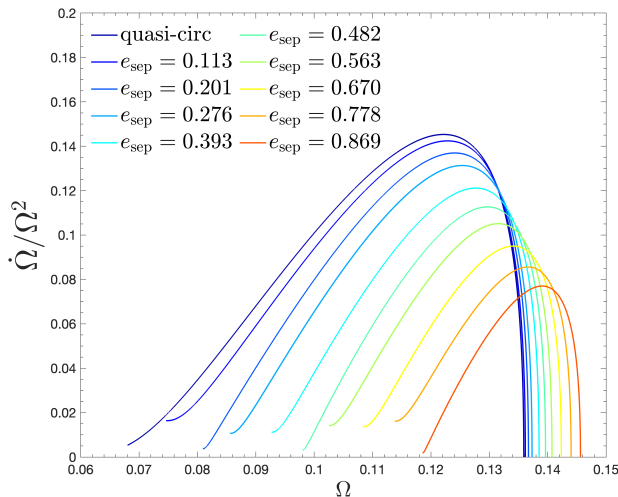
FIG. 3. Measure of adiabaticity, \dot{\Omega}/\Omega^2 , for the quasi-circular case and different eccentric configurations. The horizontal axis is restricted between \Omega_{\dot{r}=0} and \Omega_{\text{pk}} .
