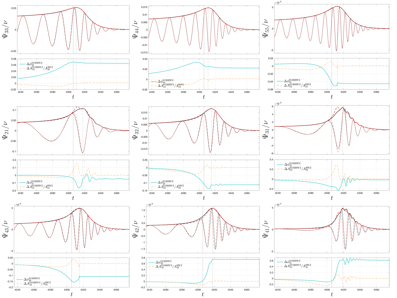
FIG. 10. Quasi-circular configuration, higher modes, EOB/RWZ comparisons. The vertical solid black lines mark t_{A_{\ell m}}^{\text{peak}} , while the dash-dotted ones mark t_{A_{\ell m}}^{\text{peak}} . Bottom panels: relative amplitude difference (orange, dashed) and phase difference (light blue). For each mode, the NQC corrections are determined according to the best prescription selected in Fig. 9.
