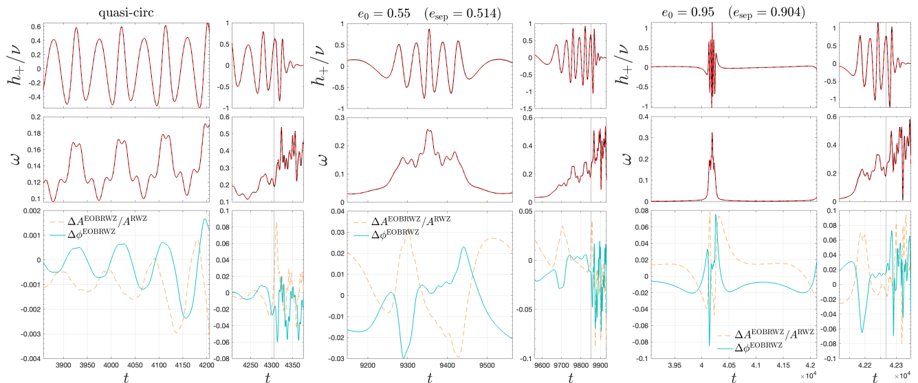
FIG. 13. EOB (red dashed) versus RWZ (black, solid) strain comparison for e_0 = \{0, 0.55, 0.95\} . The direction is (\Theta, \Phi) = (\pi/4, 0) and all modes with m > 0 are summed up to \ell = 4 , plus the (5,5) one. Bottom panels: relative amplitude difference and phase difference (in radians). The vertical lines mark the peak of the quadrupolar amplitude.
