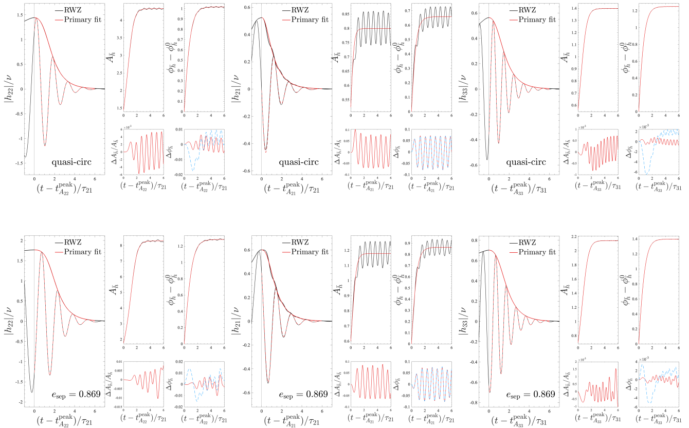
FIG. 5. Numerical waveform (black) and postpeak primary fits (red) for the (2,2), (2,1) and (3,3) modes for the quasi-circular configuration (top row) and the configuration with e_0 = 0.9 (bottom row). We show the waveform h_{\ell m} and its amplitude together with the QNM-rescaled amplitude A_{\bar{h}} and phase \phi_{\bar{h}} . In the two small bottom panels we show the fit/numerical relative difference for the rescaled amplitude and the difference for the rescaled phase (red). Here \phi_{\bar{h}}^0 is the phase of \bar{h} at \tau = 0 , and \tau_{\ell 1} = 1/\alpha_{\ell 1} is the QNM-damping time of the fundamental mode. We also show the RWZ/primary phase difference obtained imposing the condition c_2^\phi = \Delta\alpha_{21} in the primary fit (dashed blue).
