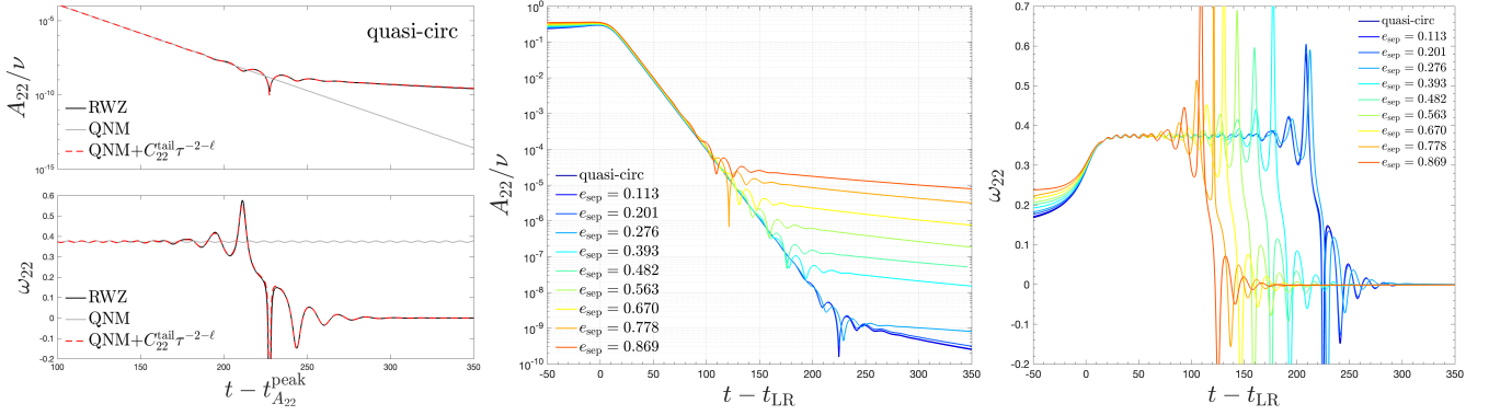
FIG. 19. Leftmost panel: Amplitude and frequency of the Zerilli (2,2) of the quasi-circular waveform (black) compared with the results obtained considering only the QNMs contribution (gray) and the QNMs plus tail (dashed red). Middle and rightmost: RWZ amplitudes and frequencies for different eccentricities, aligned with respect to the light-ring crossing.
