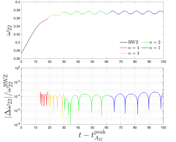
FIG. 17. Iterative QNM-fit of the frequency considering the first 4 QNMs. In the upper panel we show the RWZ frequency (black) and the results obtained with the fits. Each color represents an iteration (and thus a QNM) of the fit. In the bottom panel we show the relative difference between the fit and the corresponding n -fit. See Sec. VB for more detail on the fitting procedure.
