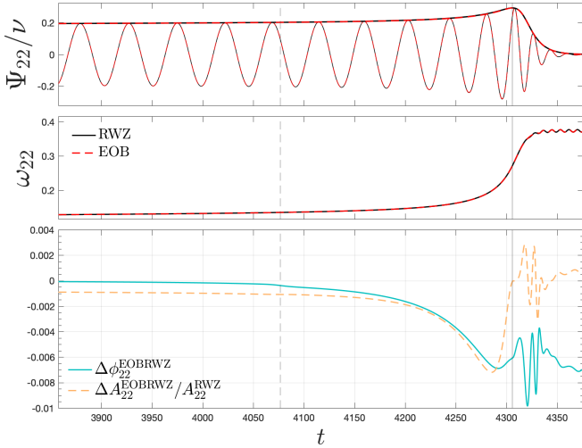
FIG. 7. Quasi-circular case, \ell = m = 2 mode: RWZ waveform (black) compared to the complete EOB one (red, dashed). The vertical lines mark the LSO crossing and the peak of A_{22} . The bottom panel shows the relative amplitude difference (dashed orange) and the phase difference in radians (solid light blue). Non-circular corrections to the waveform up to 2PN are included.
