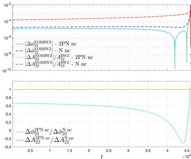
FIG. 8. EOB/RWZ phase differences (radians) and relative amplitude differences for the (2,2) mode of a quasi-circular inspiral starting from r_0 = 9 . In the upper panel we show the differences obtained with the waveform with non-circular corrections up to 2PN (solid, light blue for the phase and orange for the amplitude), and the ones obtained considering only the generic Newtonian prefactor (dashed, blue for the phase and red for the amplitude). In the bottom panel we show the ratios of these differences.
