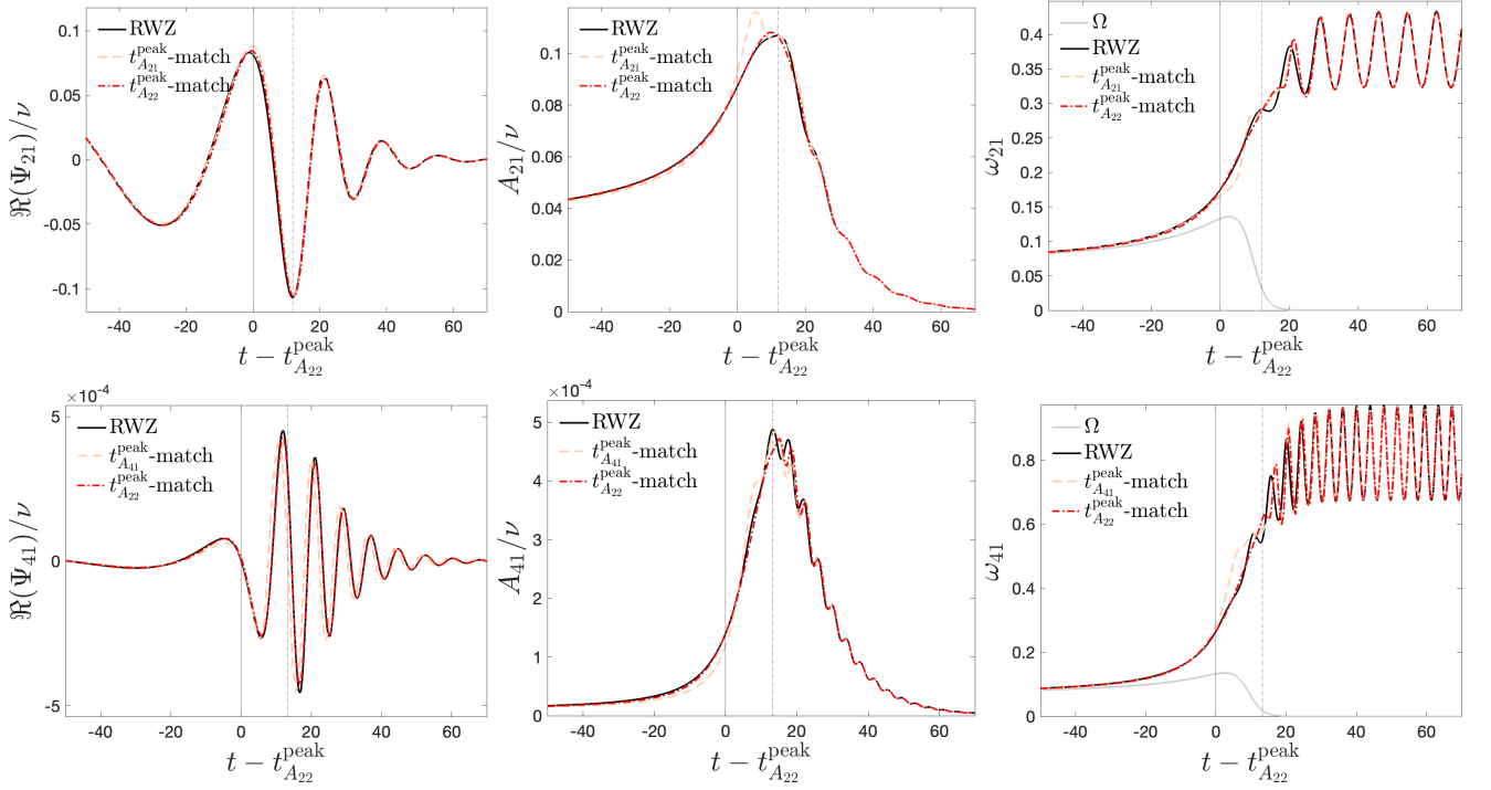
FIG. 14. Nonspinning case. New ringdown (red dashed) contrasted with the standard one discussed above (orange, dashed) for the (2, 1) and (4, 1) modes. The RWZ ringdown waveform is fitted from t_{A_{22}}^{\text{peak}} (solid vertical lines) rather than from t_{A_{\ell m}}^{\text{peak}} (dash-dotted vertical lines). This ensures a more accurate waveform description around t_{A_{\ell m}}^{\text{peak}} .
