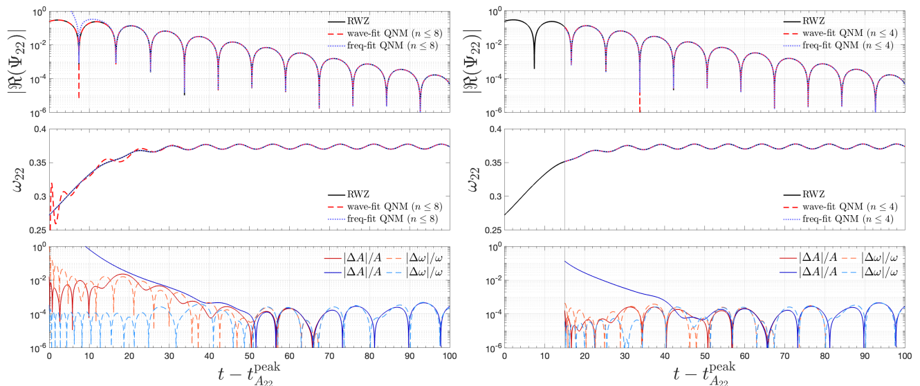
FIG. 23. Upper panels: RWZ waveform and frequency (black) compared with the results from the wave-fit (red) and frequency-fit (blue). In the bottom panels we show the relative differences of the amplitude and frequency (hot colors for the waveform-fit, cold colors for the frequency-fit). On the left, we fit the whole postpeak waveform using 8 QNMs, while on the right we fit from t \geq 15 + t_{A_{22}}^{\text{peak}} using 4 QNMs. See discussion in Appendix B.
