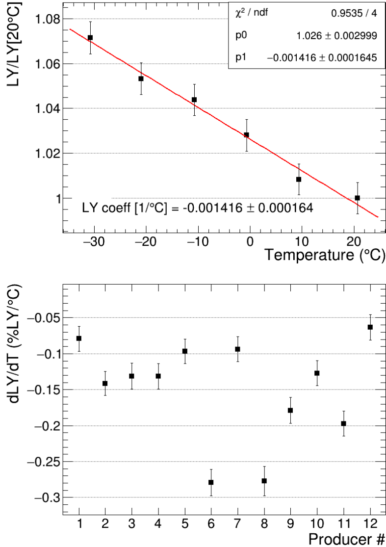
Figure 19. (top) LY normalized to the corresponding value at T = 20^{\circ}\text{C} as a function of the temperature. The normalized LY error bars were determined by propagation of the measurement uncertainties. From the linear fit, the LY temperature coefficient is obtained. (bottom) Light yield temperature coefficient for the 12 producers. The error bars correspond to the fit uncertainties.
