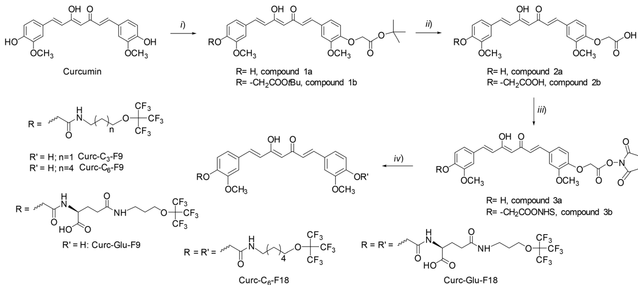
Scheme 2 Synthesis of mono and bis-perfluorinated curcumin derivatives: (i) t -butyl bromoacetate, K 2 CO 3 in CH 3 CN; (ii) TFA/CH 2 Cl 2 (1:1); (iii) EDC/NHS, 5 mol% DMAP in NMP; (iv) F9-C 3 -NH 2 or F9-C 6 -NH 2 or F9-Glu-NH 2 , buffer phosphate (0.1 M, pH = 7.5), CH 3 CN.
