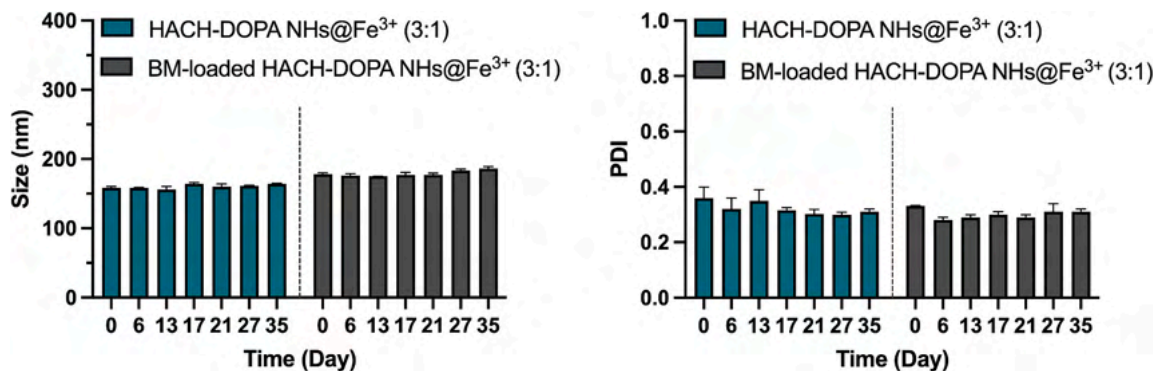
Fig. 6. The mean diameter and PDI of Fe 3+ modified HACH-DOPA nanogels and drug-loaded nanogels (DL% ~15 %) as a function of time at 4°C. All the data are expressed as the mean value ± standard deviation. Results were obtained in triplicate (n = 3).
