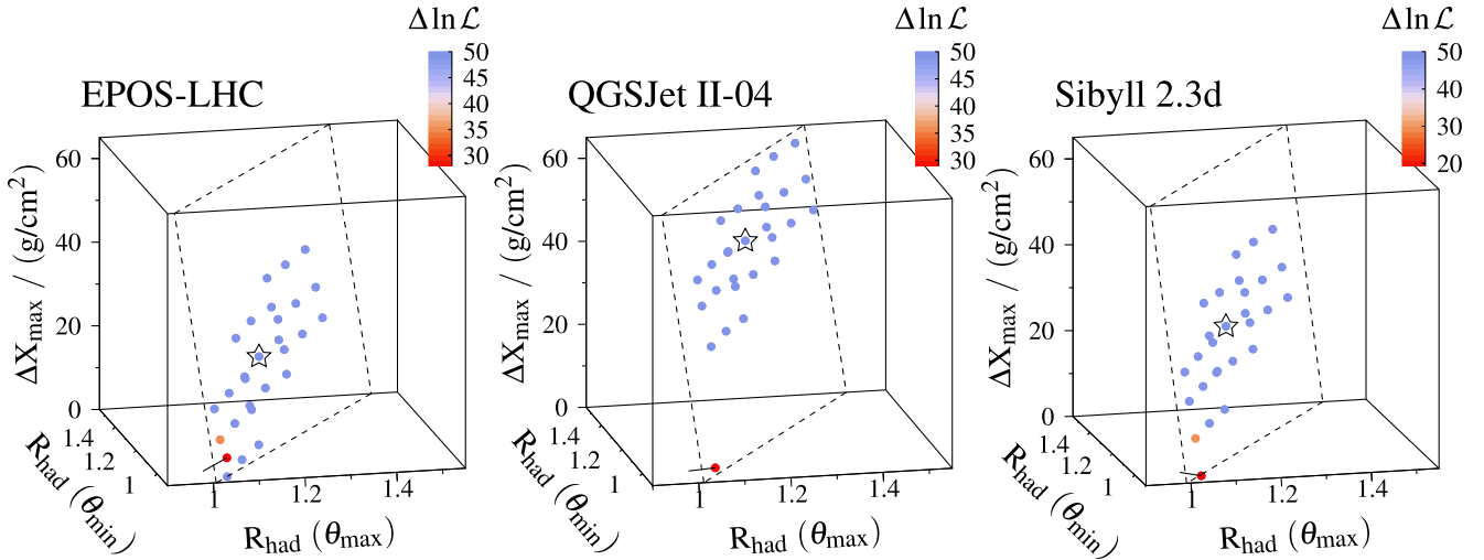
FIG. 9. Values of the modification parameters (points) for all possible combinations of experimental systematic uncertainties on the energy ( \pm 14\% ), X_{max} ( \pm_9^8 \text{ g/cm}^2 ), and S(1000) ( \pm 5\% ). The color of the points shows the difference in log-likelihood expressions ( \Delta \ln \mathcal{L} ) in the case of no modifications and in the case of the assumed template modifications, including the differences higher than 50 (note the slightly different scale between models). The results (see Table III) for no systematic shift of the data are highlighted by stars. Dashed lines outline the contour of the plane from the best-fit to the points. The closest approach to the nonmodified ( R_{had}(\theta) = 1 , \Delta X_{max} = 0 \text{ g/cm}^2 ) model predictions using a dense scan of linear combinations of experimental systematic uncertainties is connected with this point by a black line. The animated rotated views are available at [40].
