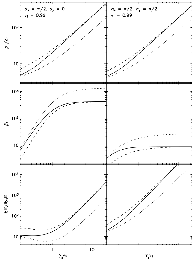
Figure 5. Density contrast (top), plasma \beta (middle) and magnetic field strength (bottom) for v_t = 0.99 . The magnetic field is purely transverse and aligned with the tangential component of velocity on the left-hand side, while it is orthogonal on the right-hand side. Different lines have the same meaning as in Fig. 2.
