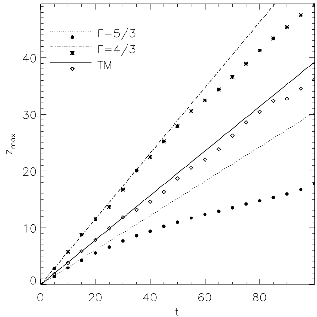
Figure 10. Position of the working surface as a function of time for \Gamma = 5/3 (circles), \Gamma = 4/3 (stars) and the TM EoS (diamonds). Solid, dotted and dashed lines gives the one-dimensional expectation.
