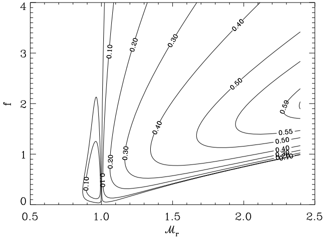
Fig. 3. Same as Fig. 1, but for \zeta = 1 .
