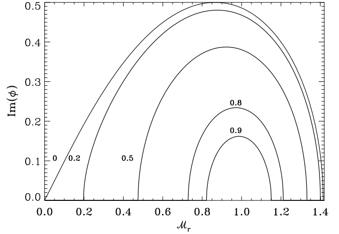
Fig. 4. Dependence of \text{Im}(\phi) on the relativistic Mach number for fixed \beta = 10^{-3} and f = 0 ( \Gamma = 5/3 ). The different labels above each curve indicate the values of the Alfvén Mach number \zeta = [0, 0.2, 0.5, 0.8, 0.9] .
