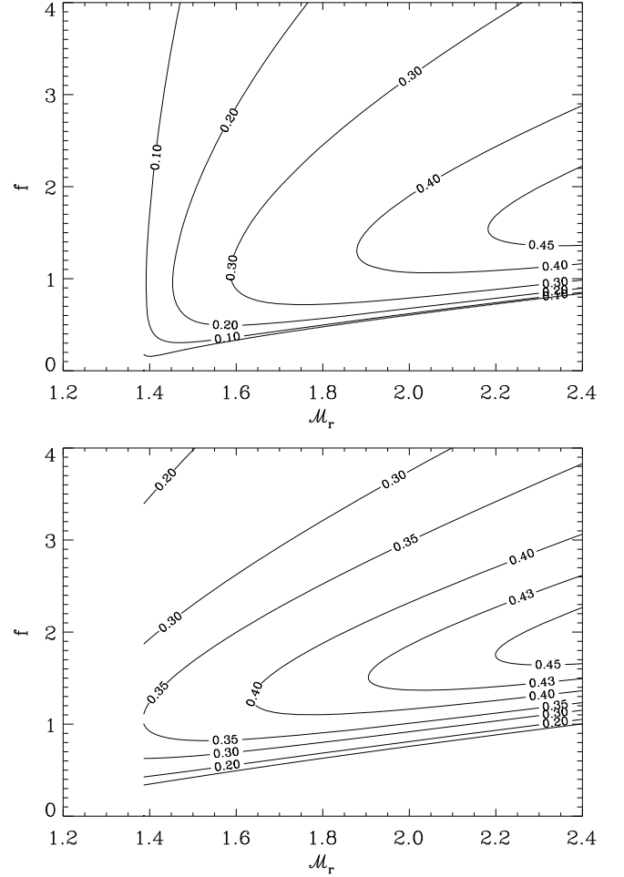
Fig. 7. Contour plots of constant \text{Im}(\phi) lines in the M_r - f plane for \beta = 0.7 , \zeta = 1.2 ( top panel ) and \zeta = 1 ( bottom panel ). Here \Gamma = 4/3 was used.
