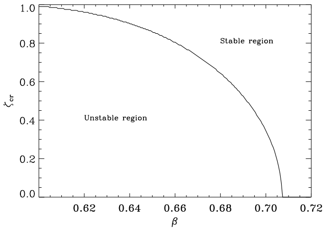
Fig. 9. Effect of the kinematic factor on the instability when f = 0 ( \Gamma = 4/3 ). As is clear, for \beta \approx 0.71 the instability is suppressed by relativistic effects independently of the value of M_r .
