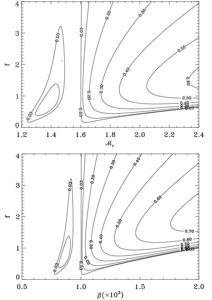
Fig. 1. Two contour plots are shown. Top panel: the contour plot of constant \text{Im}(\phi) surfaces as a function of the inclination factor f and relativistic Mach number \mathcal{M}_r for fixed Alfvénic Mach number \zeta = 1.6 and flow velocity \beta = 10^{-3} . Bottom panel: the contour plot of constant \text{Im}(\phi) surfaces as a function of the inclination factor f and \beta for the fixed Alfvén speed ( V_A = 10^{-3} ) and the sound speed ( C_s = 6.3 \times 10^{-4} ). Here \Gamma = 5/3 is used.
