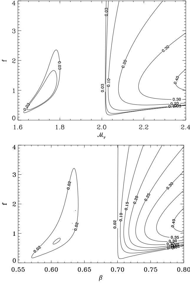
Fig. 6. Top panel: contour plots of constant \text{Im}(\phi) lines in the M_r - f plane for \beta = 0.7 , \zeta = 1.6 . The two instabilities branches are clearly visible. Bottom panel: contour plots of constant \text{Im}(\phi) lines in the \beta - f plane for V_A = 0.7 , C_s = 0.43 . Here \Gamma = 4/3 was used.
